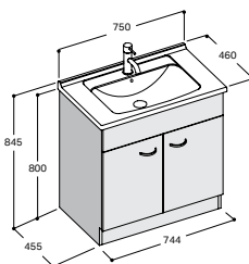
Malik Doors 750 Floor - 2 Door Mineral Cast Basin Code 51001-W (White)
