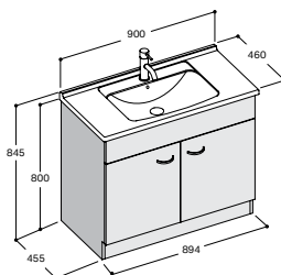
Malik Doors 900 Floor - 2 Door Mineral Cast Basin Code 51201-W (White)
