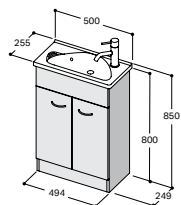
Malik Doors 500 x 250 Floor - 2 Door Mineral Cast Basin Code 30101-W (White)
