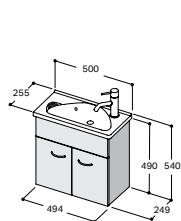
Malik Doors 500 x 250 Wall - 2 Door Mineral Cast Basin Code 31101-W (White)
