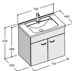
Malik Doors 750 Wall - 2 Door Mineral Cast Basin Code 33900-W (White)
