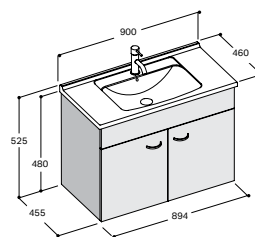
Malik Doors 900 Wall - 2 Door Mineral Cast Basin Code 34000-W (White)
