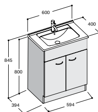
Malik Doors 600 x 400 Floor - 2 Door Mineral Cast Basin Code 30201-W (White)
