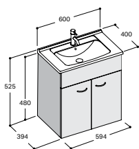
Malik Doors 600 x 400 Wall - 2 Door Mineral Cast Basin Code 31201-W (White)
