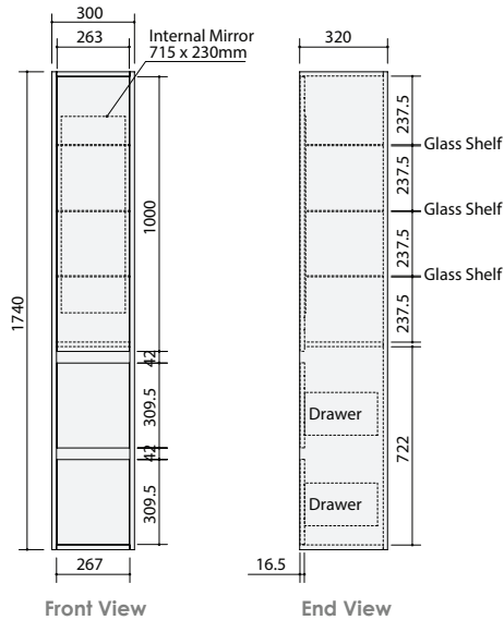
City Tower 1740 - 1 Door, 2 Drawer
