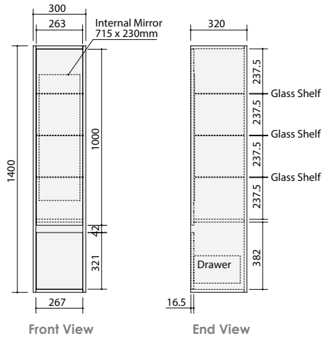
City Tower 1400 - 1 Door, 1 Drawer
