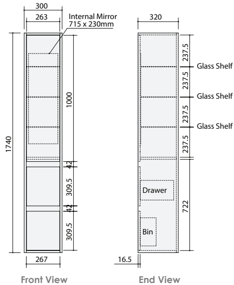
City Tower 1740 - 2 Door, 1 Drawer (with bin)
