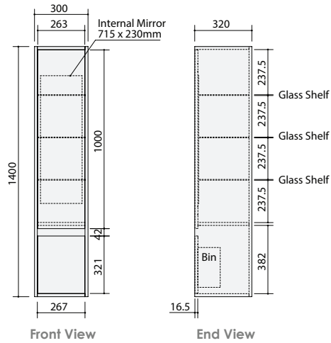
City Tower 1400 - 2 Door (with bin)
