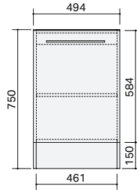
Maxi Floor 500 -1 Door (left and right hinged)
