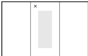
1200 Models
