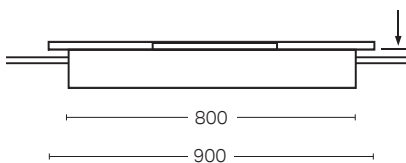
Recess Plan View
