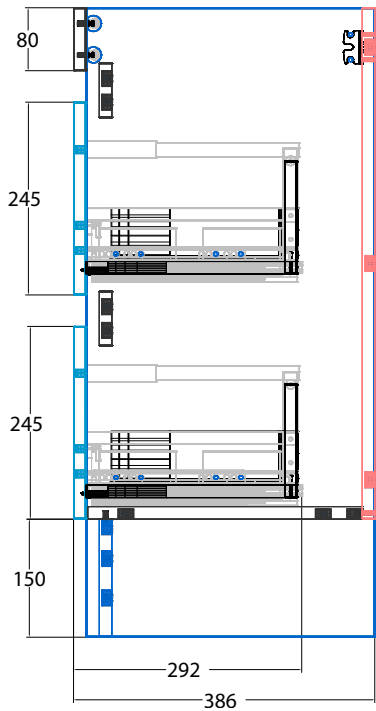
SIDE
