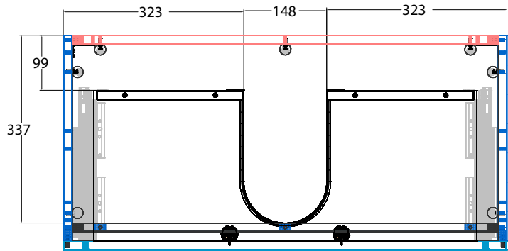
PLAN
