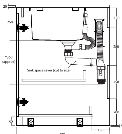
SIDE (SECTION VIEW)
