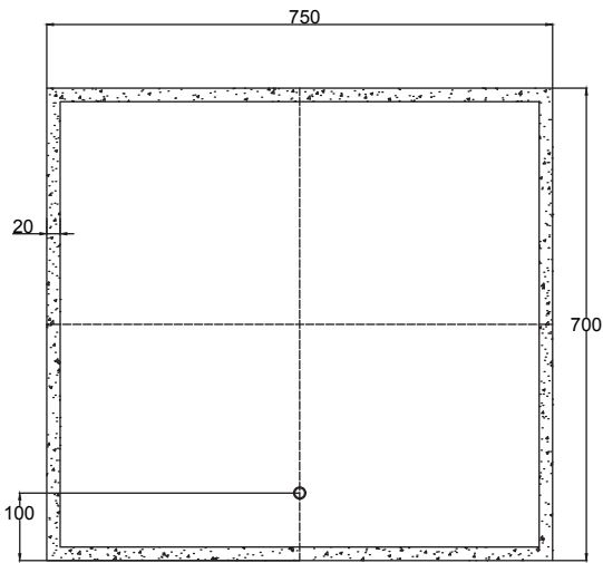
FRONT
