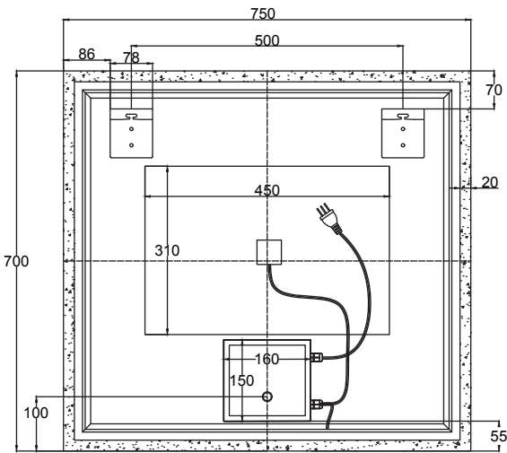
REAR
