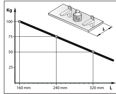
Capacity loading of the shelf
